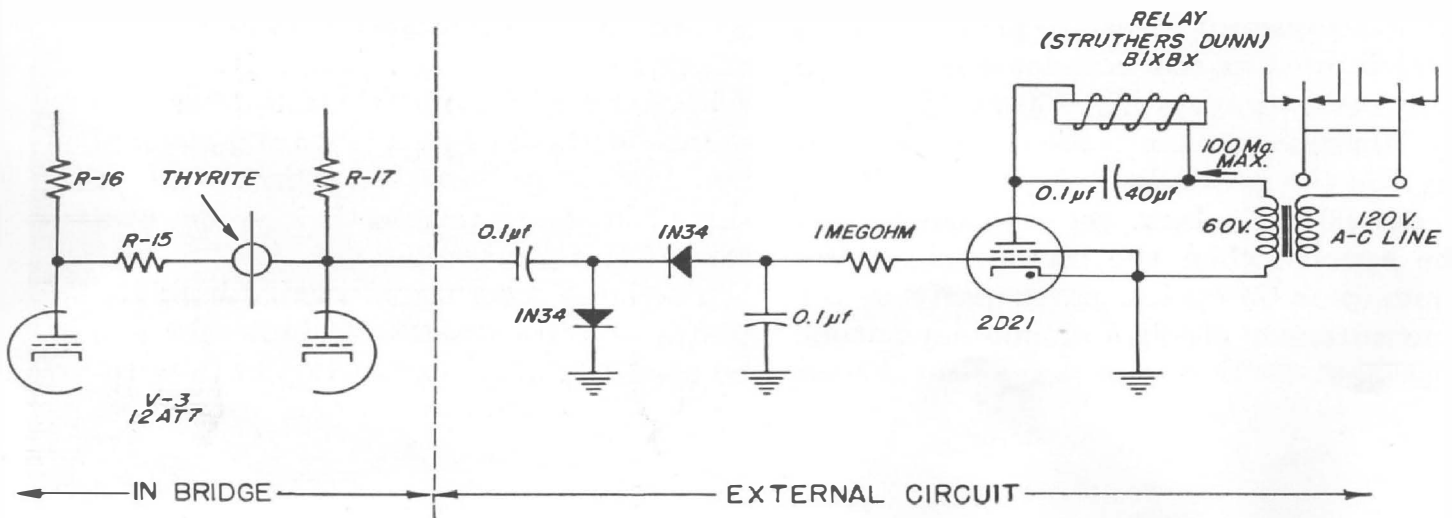
Figure 4. Simple circuit for operating automatic sorting equipment.
