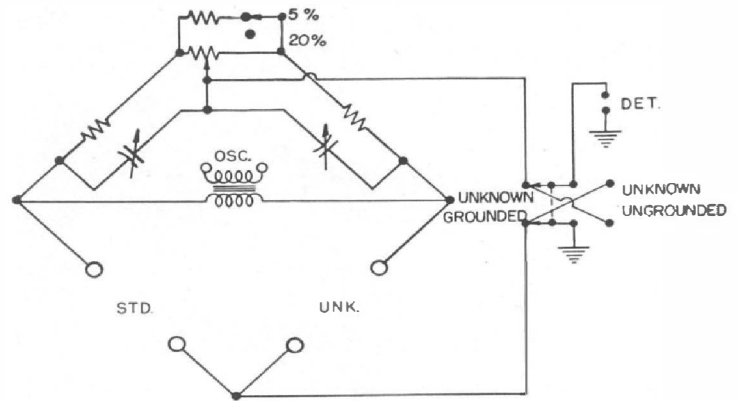
Figure 2. Elementary schematic circuit diagram of the bridge.
