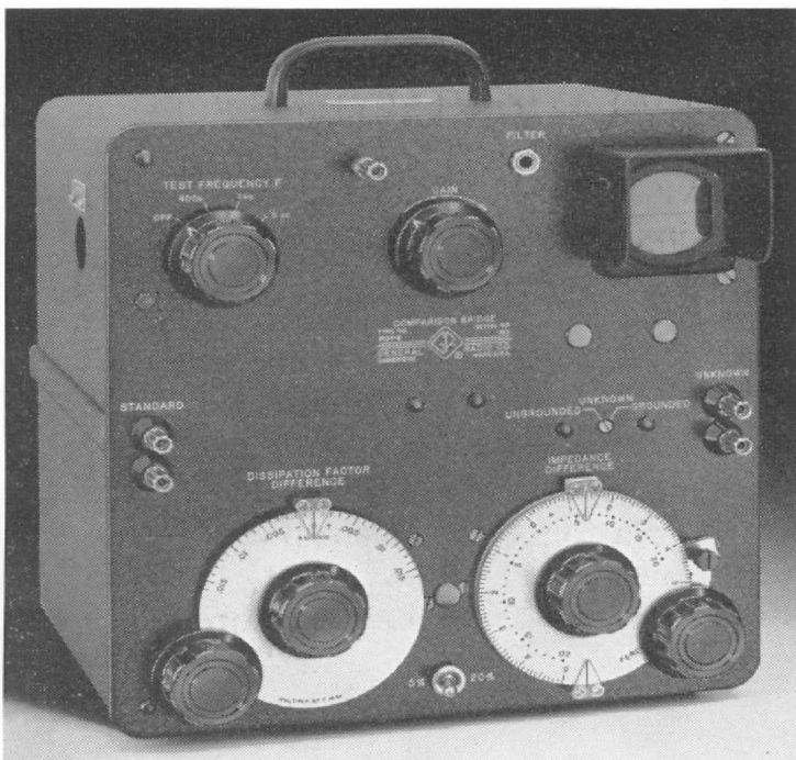
Figure 1. Panel view of the Type 1604-B Comparison Bridge.
